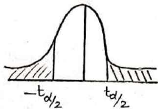
(Two-tailed Test)
